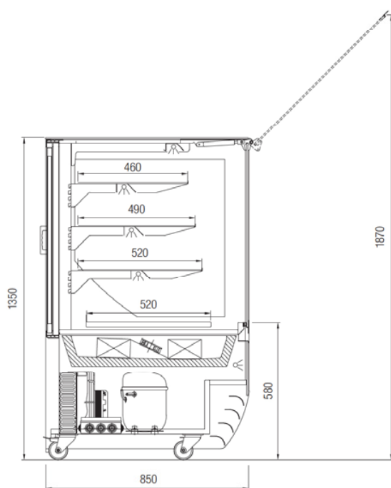
Bokorys Magnum
