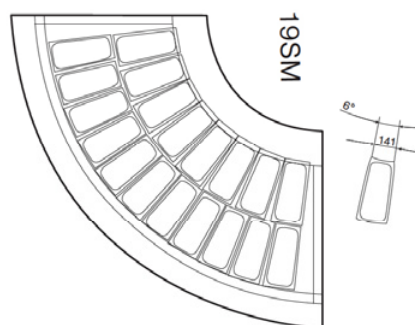
Roh MGI 19 / NZ 90 a schéma GN
