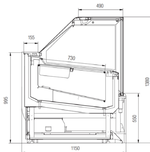
Bokorys Limosa
